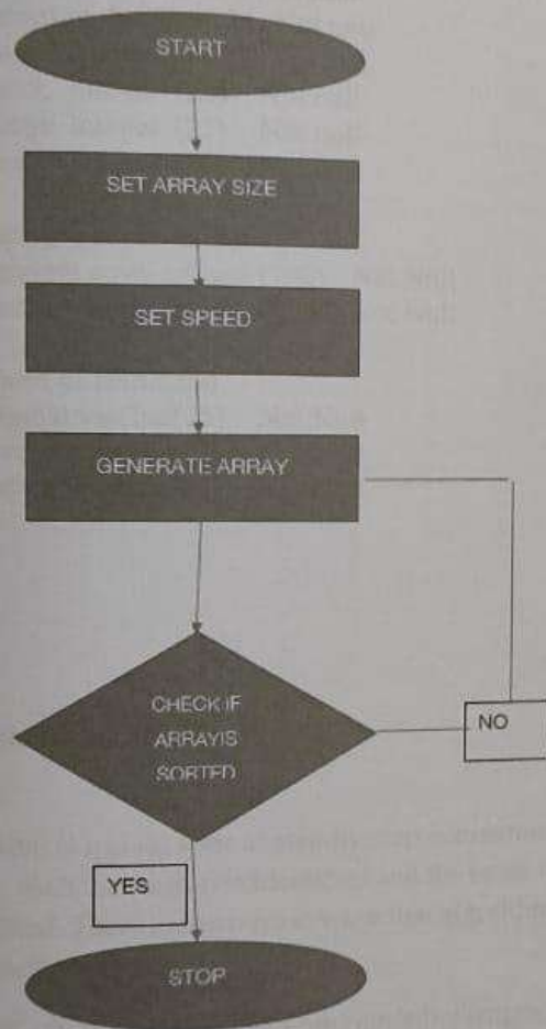
Figure 10 : Flowchart
