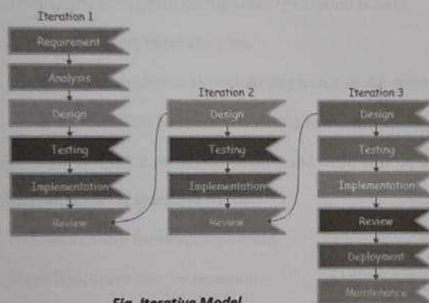
Fig. Iterative Model
